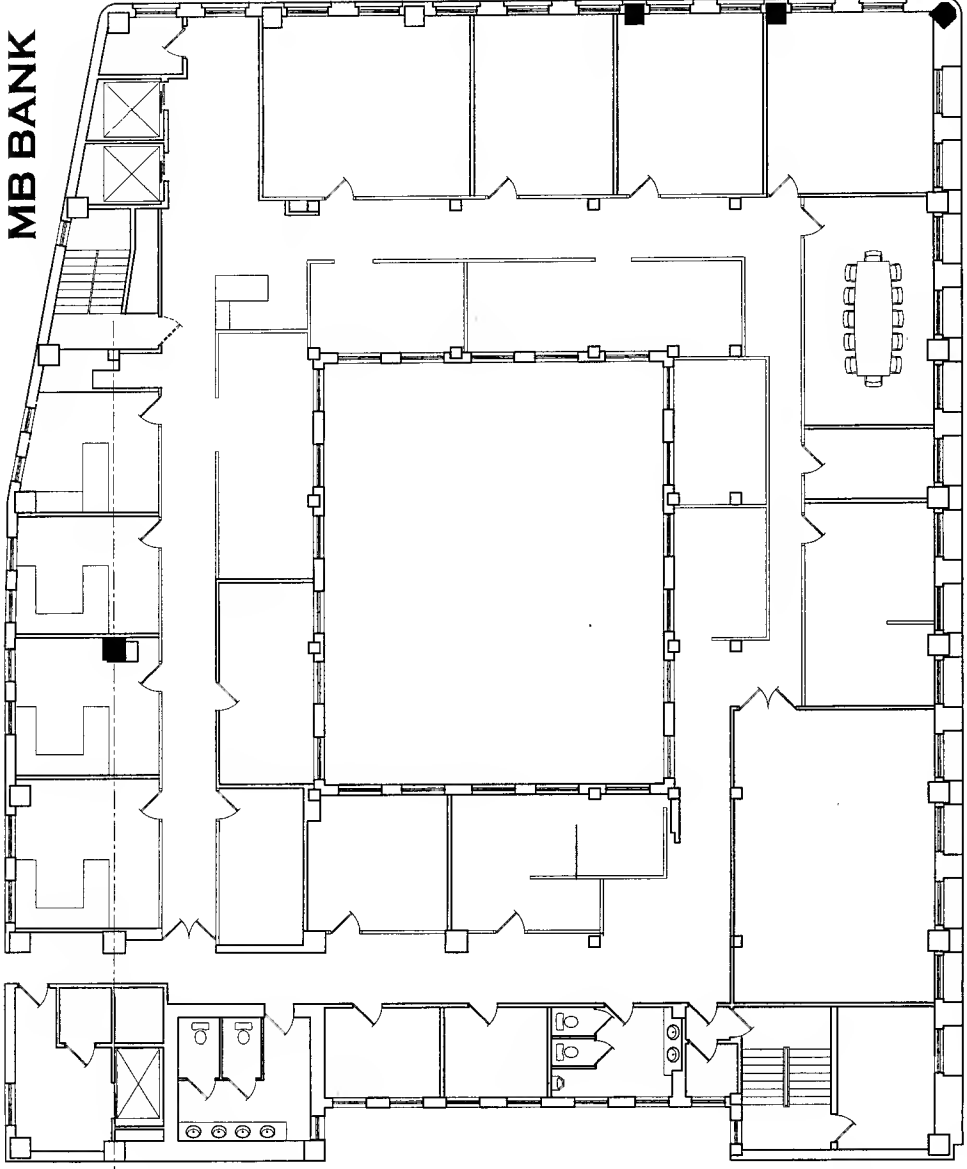
Figure 14 4-TH FLOOR PLAN
